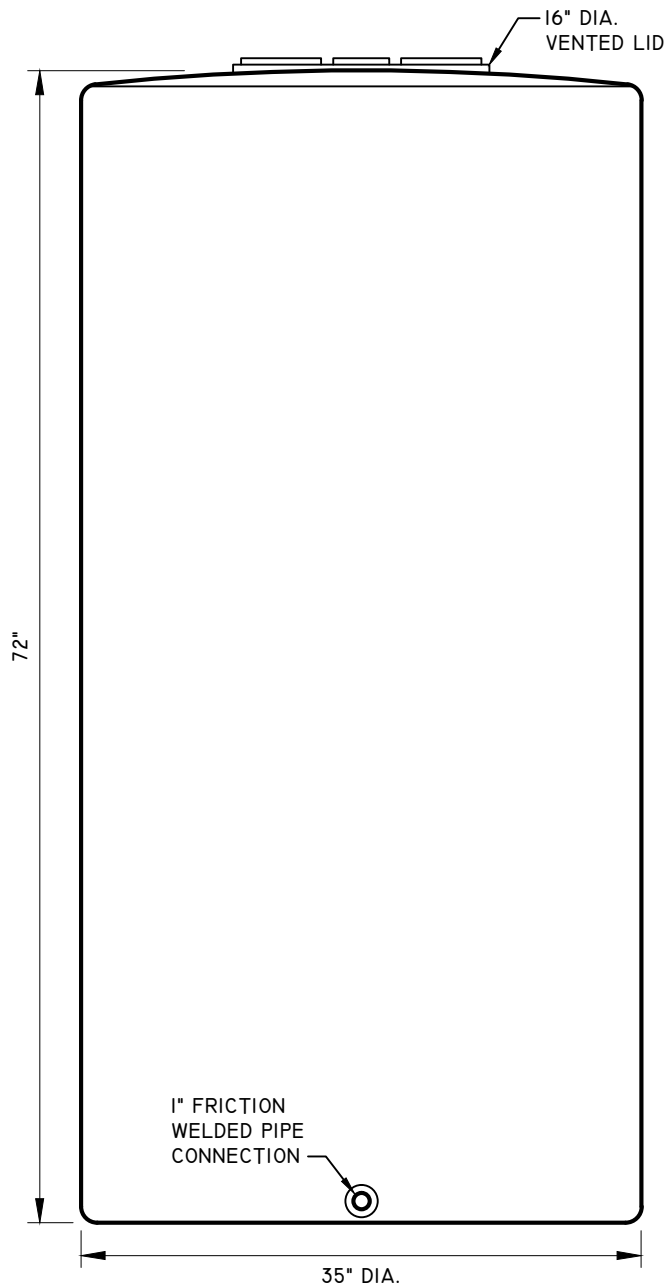
SIDE ELEVATION
