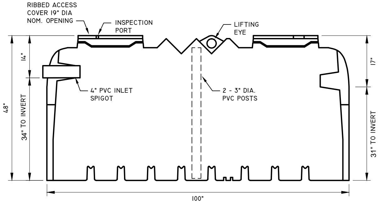
SECTION
