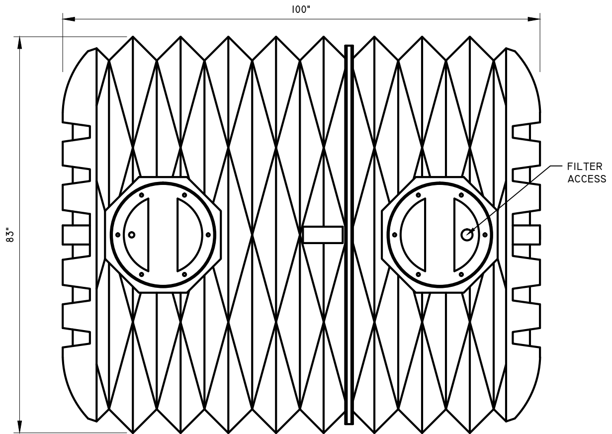
PLAN VIEW
