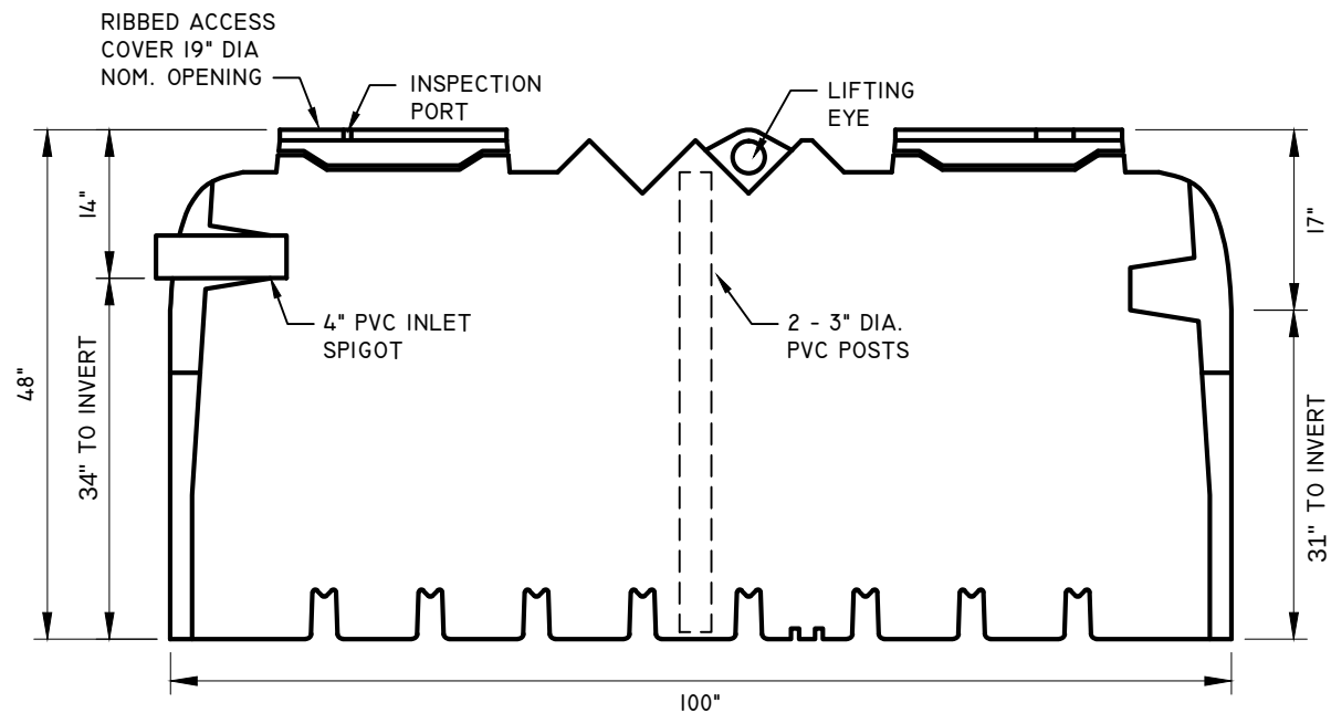
SECTION
