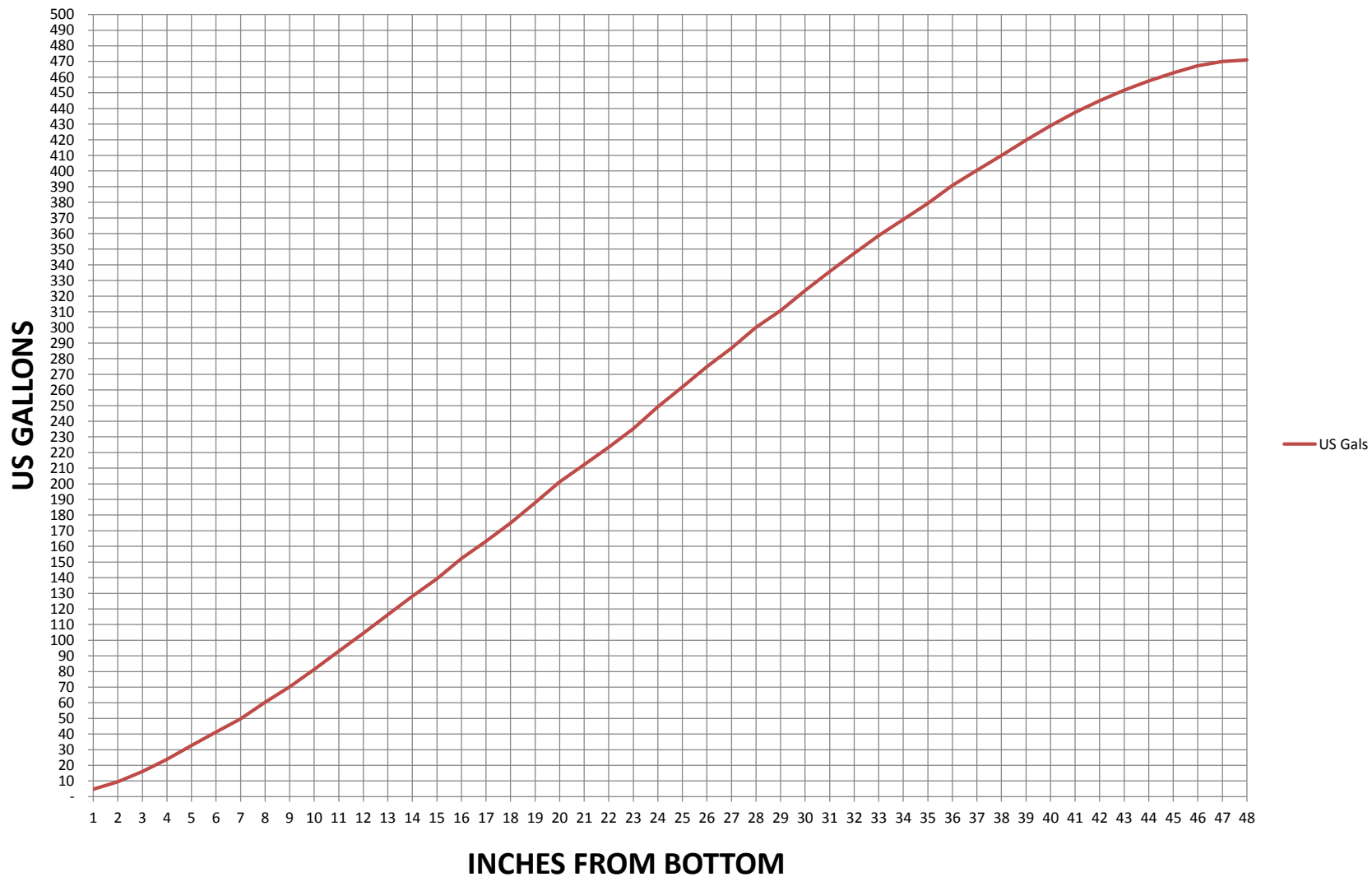
LTU 455 LEG TANK - WATER VOLUME (APPROX)
