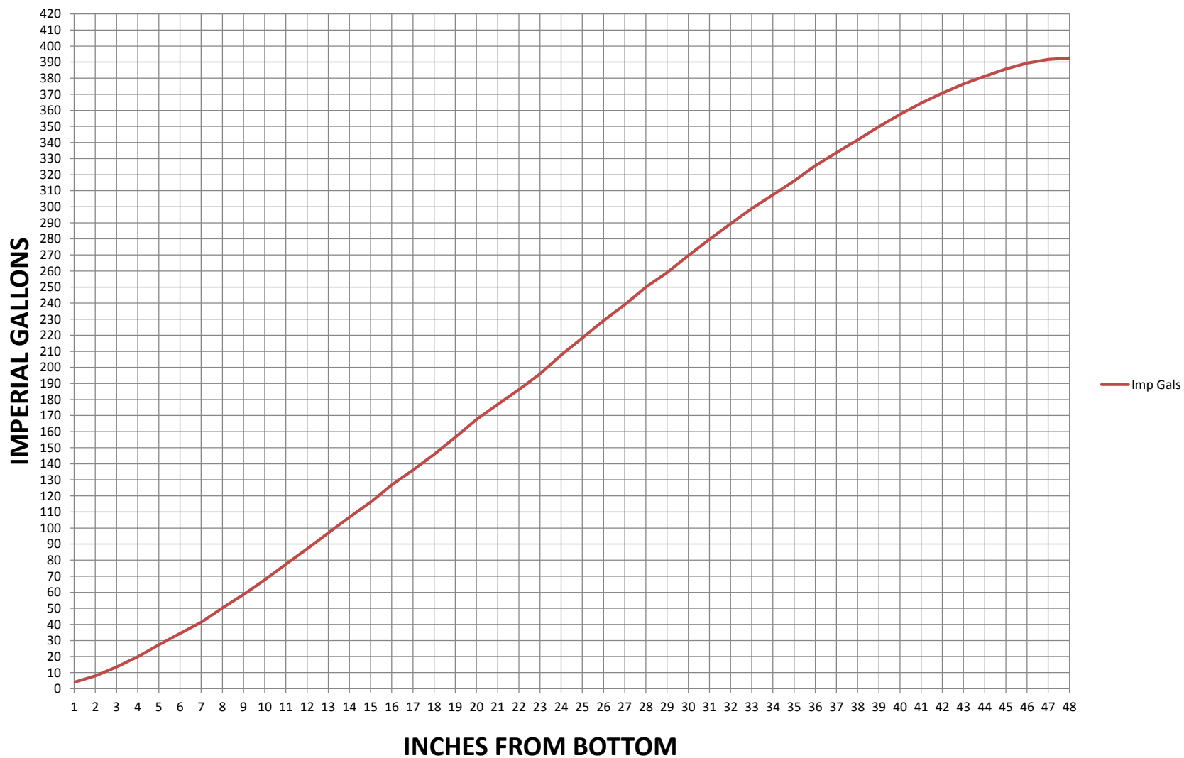
LT 380 LEG TANK - WATER VOLUME (APPROX.)
