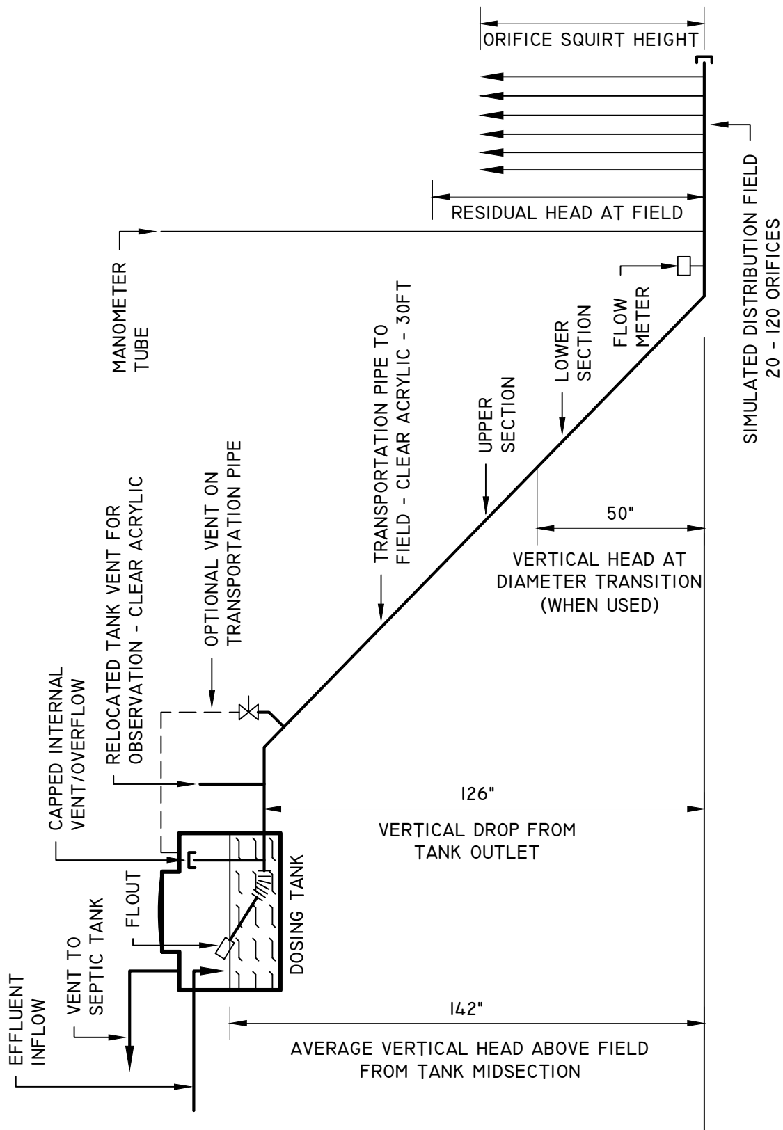
FLOUT® TEST APPARATUS
