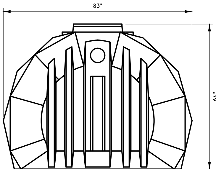
END VIEW
