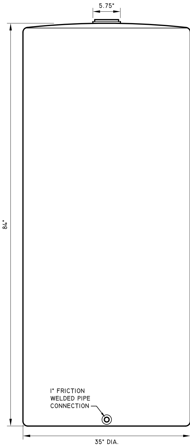
SIDE ELEVATION
