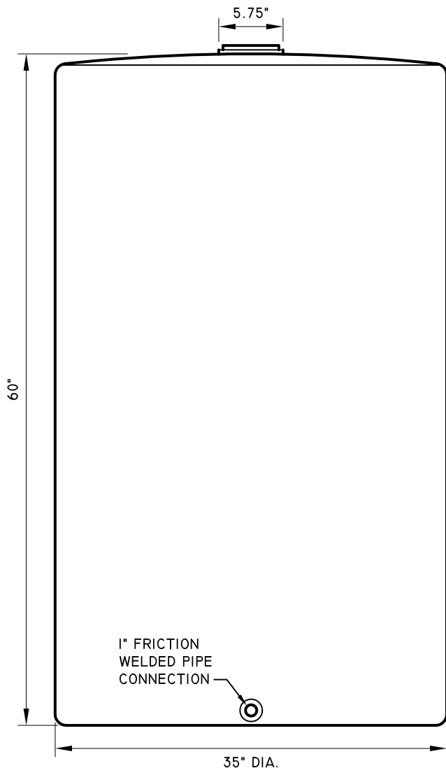
SIDE ELEVATION
