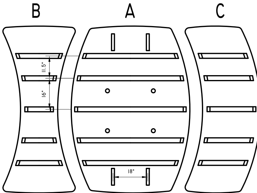
BOTTOM RIBS
