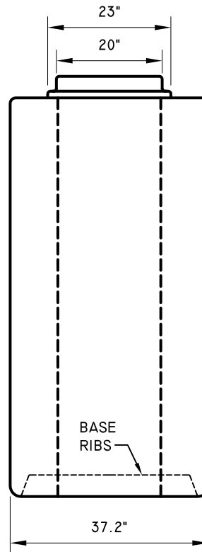
END VIEW
