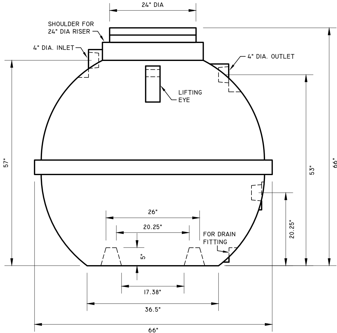
SIDE ELEVATION
